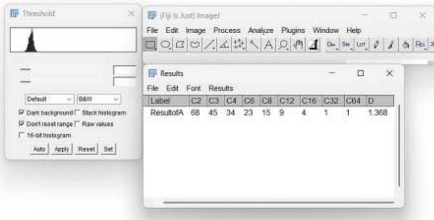
Figure 1. Fractal dimension analysis performed using ImageJ software.
